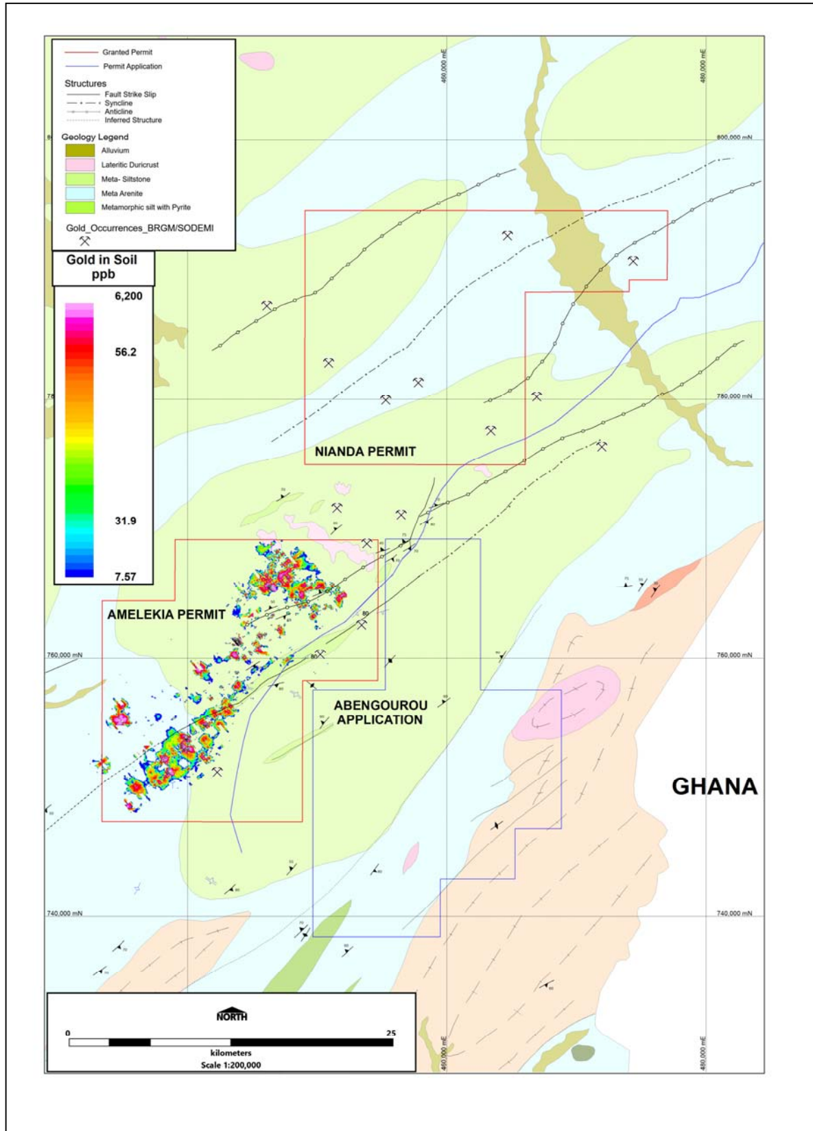
Figure 2: Abengourou Project- Highlighting District Geology with the New Nianda Permit alongside the Amélékia Permit and contiguous Abengourou Application. Historic soil sampling highlight the highly gold anomalous Amélékia permit where confirmatory sampling has begun.
