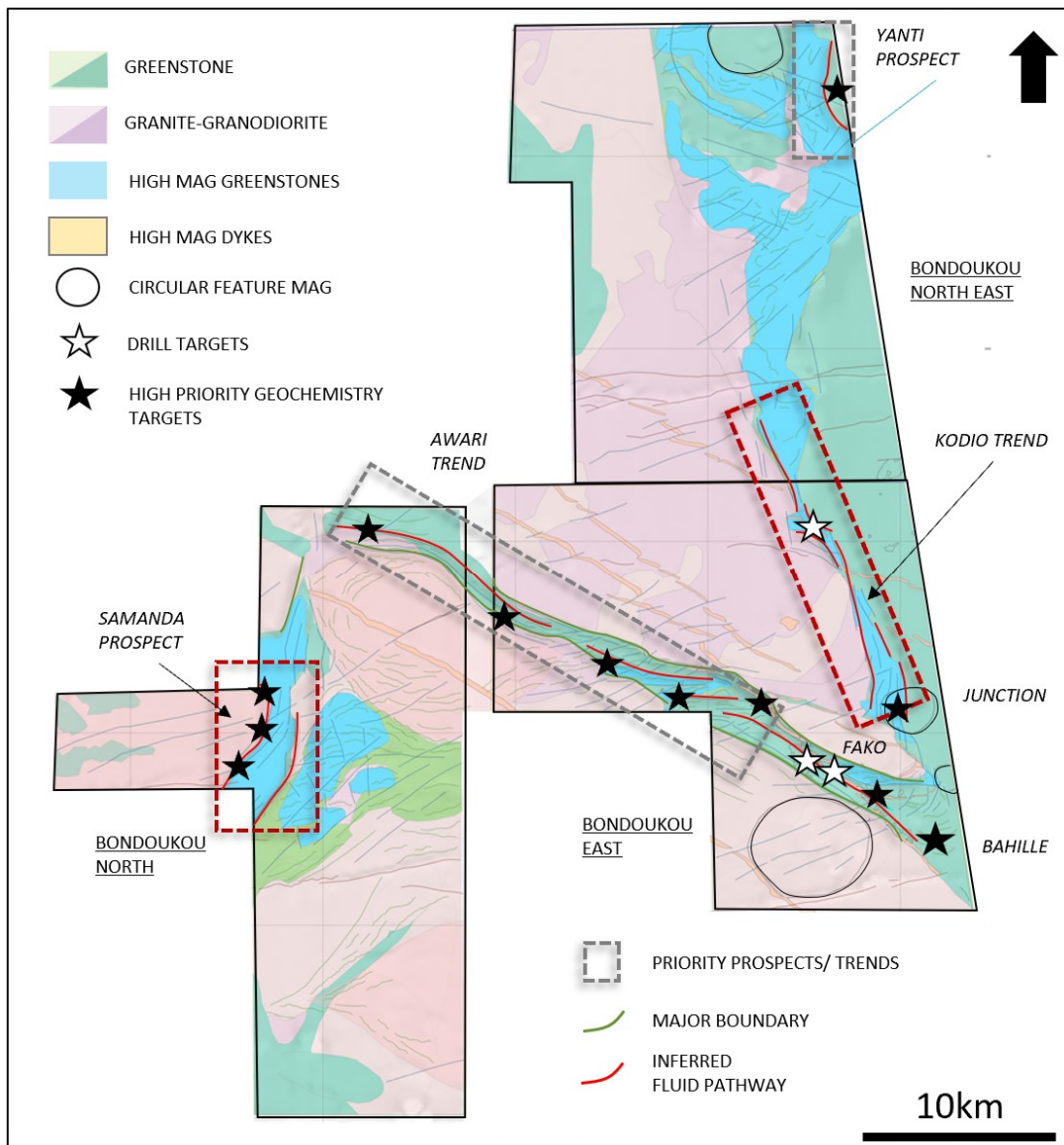
Figure 1: Bondoukou Project – Gold Target Trends/Fluid Pathways.
