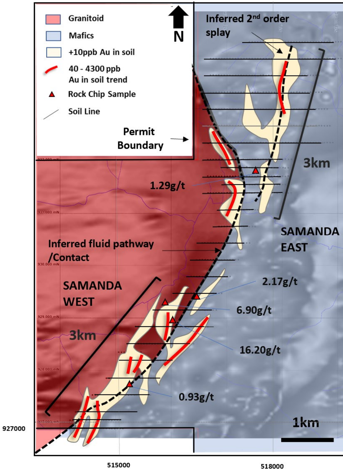
Figure 2: Samanda Soil results over greyscale magnetics and summary geology. 2 main 3km long trends defined with +40ppb cores. Best rock chip samples also depicted.
