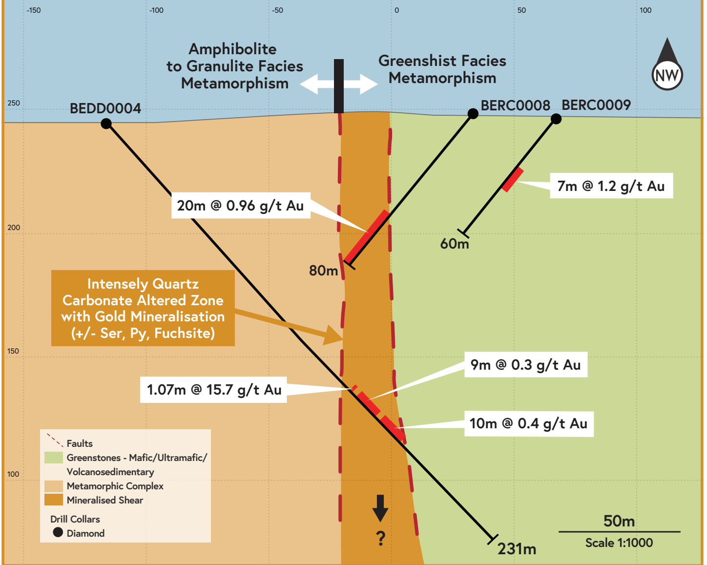
Fako/Fako South Cross Section A/A' BEDD004 – Looking NW
