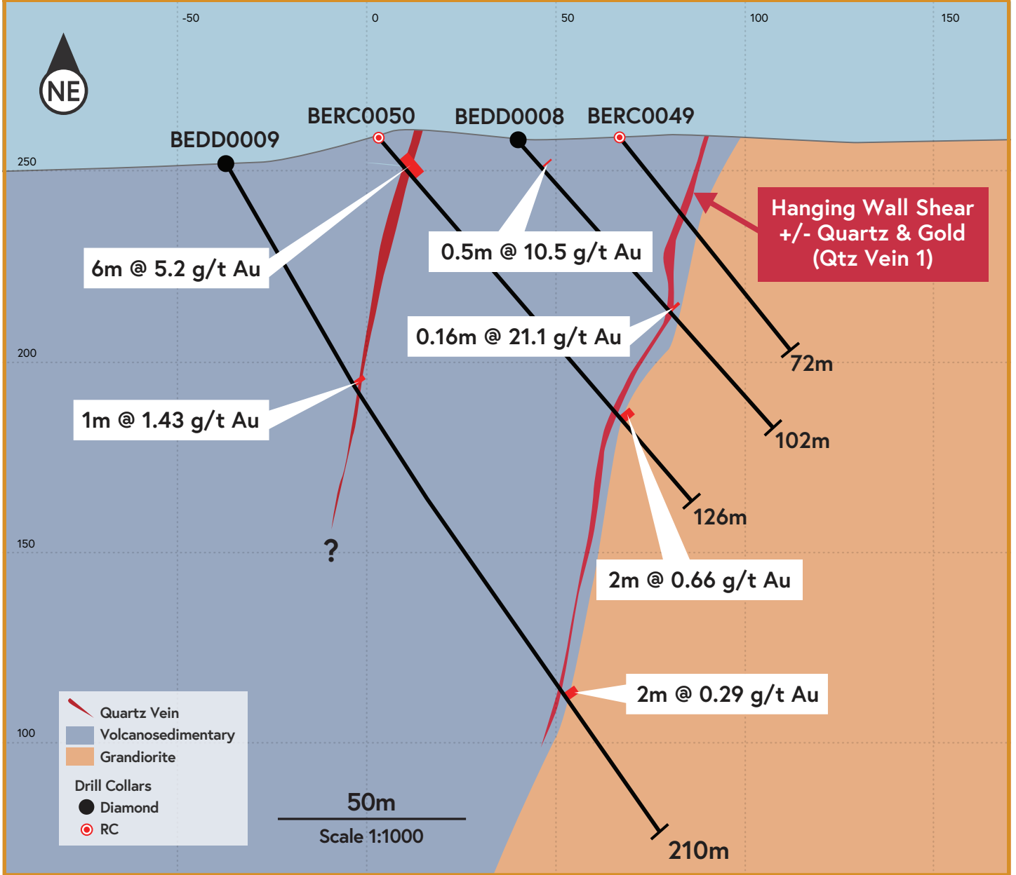
Casino Cross Section – B-B' Looking NE
