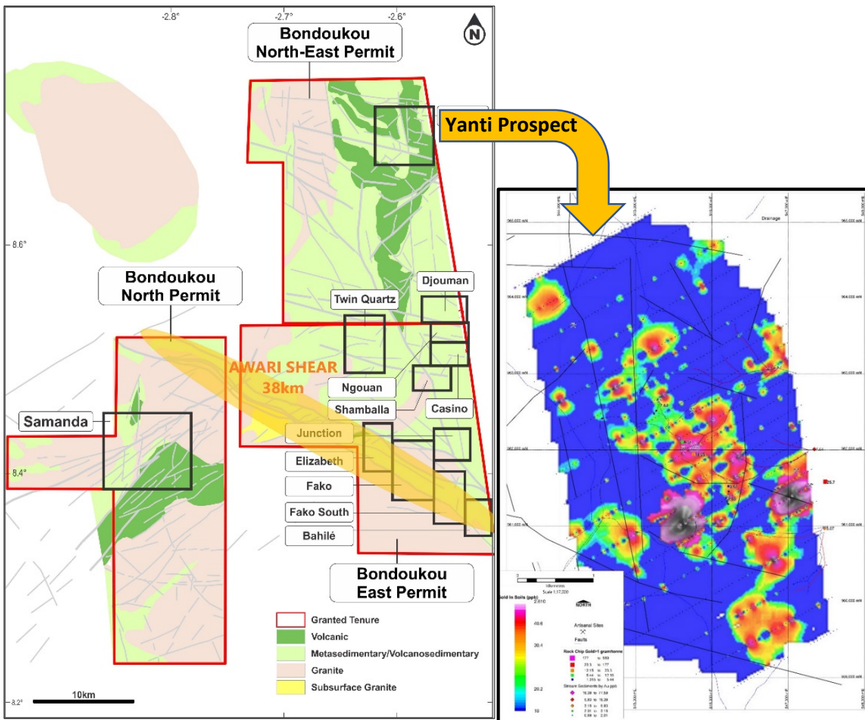
Figure 2: Bondoukou Project prospect locations and gridded soil results for the Yanti prospect.
